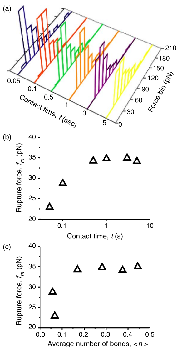
Fig. 4. Dependence of rupture force on contact duration. (a) Histograms of rupture forces measured at the indicated contact durations. Total of > 100 forces at each contact time (except at t = 0.05 s, which had \sim 50 forces) were collected and analyzed by histogram of bin size of 15 pN. (b) Dependence of the most probable rupture force, f_m (open triangles), on contact durations. (c) Correlation between most probable force f_m and average number of bonds, \langle n \rangle = -\ln(1 - P_a) , calculated from Eq. (1) [38]. The approach and retraction velocities were v_a = v_r = 1000 \text{ nm/s} .
